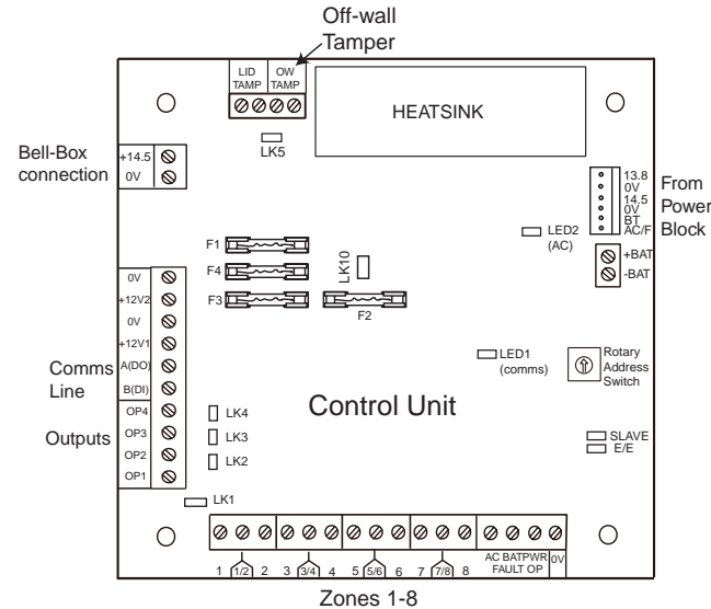
Figure 1. Control Unit
