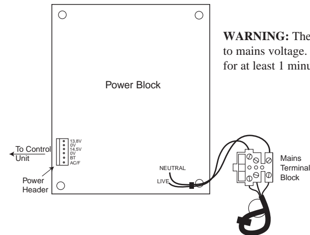
Figure 2. Power Block
