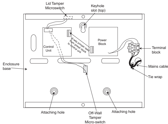
Figure 3. Enclosure Base
